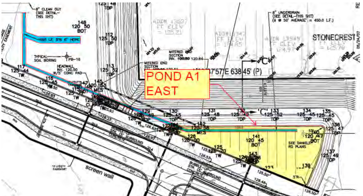
Site plans of pond; Details of underdrain system
